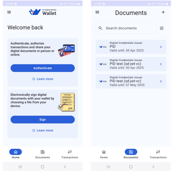
(a) EUDI home screen
