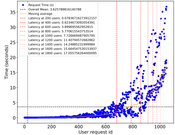
Fig. 9: Latency with up to 2000 users
