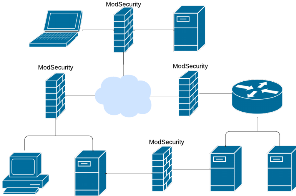
Fig. 2: TrustZero architecture overview
